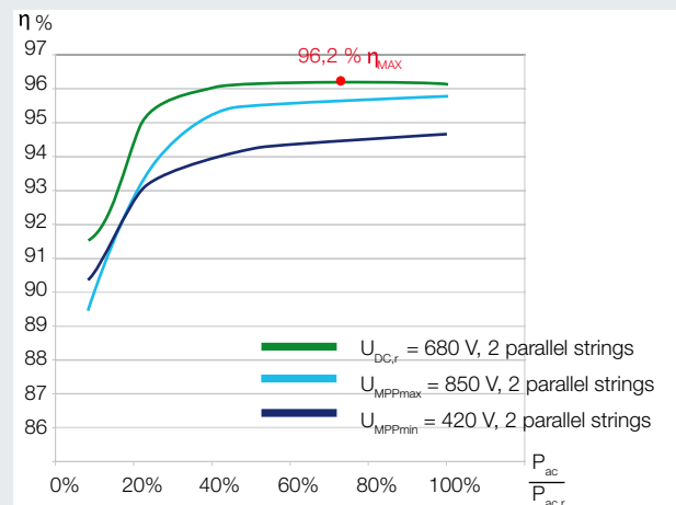
Efficiency rate characteristic curves PIKO 10.1
