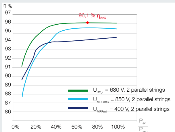
Efficiency rate characteristic curves PIKO 8.3
