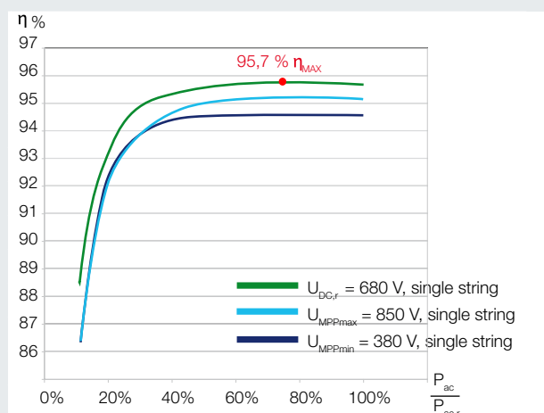
Efficiency rate characteristic curves PIKO 3.0
