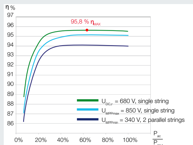
Efficiency rate characteristic curves PIKO 3.6
